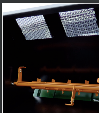
Perforated metal sheet and bolted folded sections on the top agitator
