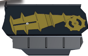
Hydraulic agitator system to prevent bridging
