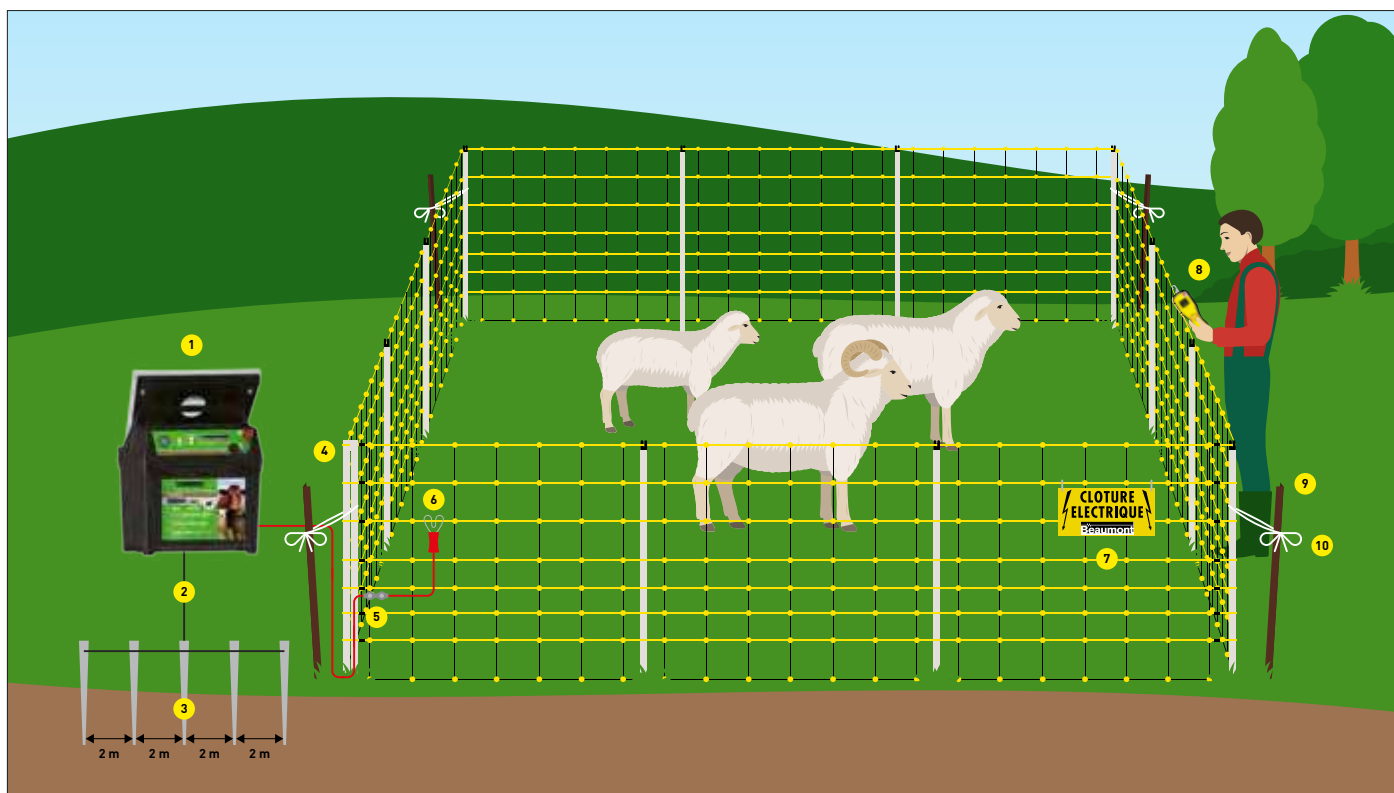
DIAGRAM OF MOBILE FENCING FOR SHEEP
