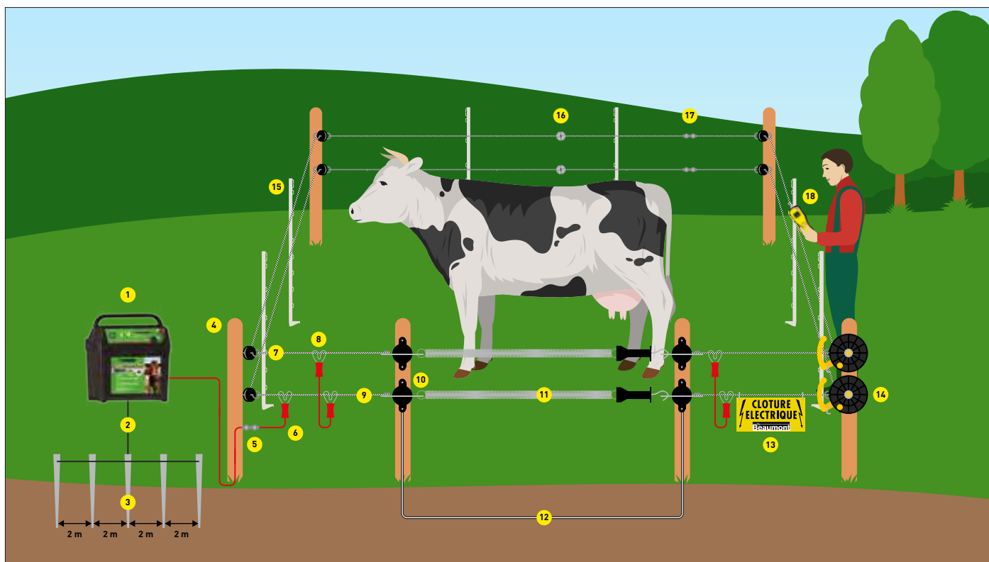
DIAGRAM OF MOBILE FENCING FOR COWS
