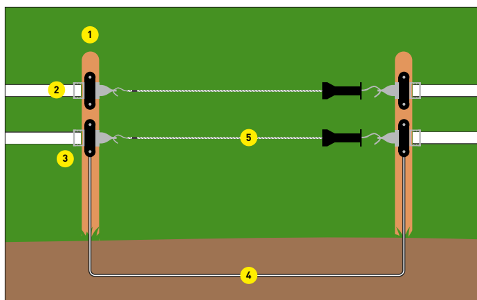
DIAGRAM OF GATE KIT
