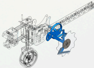
Leaf protection discs
