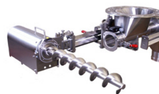
Dosing screw with drive, extracted and swivelled to the side.
