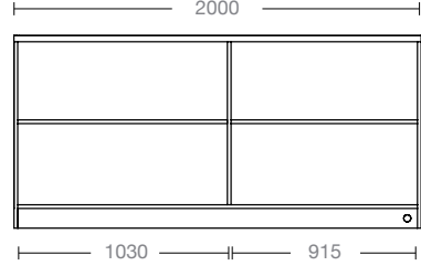
BANCO BAR NEUTRO L2000 H950 P825MM AMBIENT BAR COUNTER W2000 H950 P825MM
