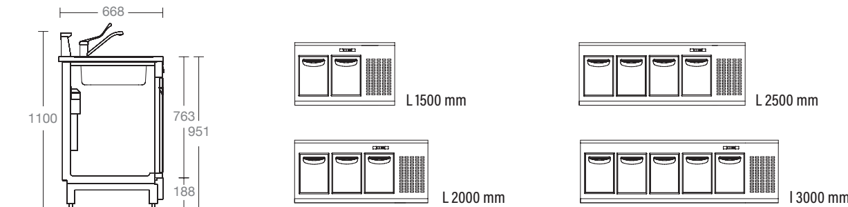
BASE CON CELLE REFRIGERATE STATICHE E MOTORE INCORPORATO H1100 P668 MM BACK-BASE WITH STATIC REFRIGERATED ROOMS & HERMETIC UNIT H1100 D668
