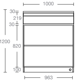
BANCO BAR NEUTRO L1000 H1200 P905MM AMBIENT BAR COUNTER W1000 H1200 P905MM
