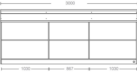
BANCO BAR NEUTRO L3000 H1200 P905MM AMBIENT BAR COUNTER W3000 H1200 P905MM
