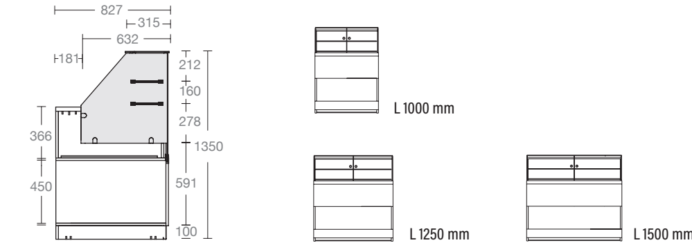
VETRINA PANETTERIA NEUTRO H1350 P825 MM BAKERY AMBIENT DISPLAY CASE H1350 D827 MM
