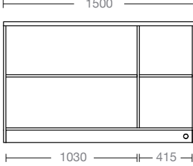
BANCO BAR NEUTRO L1500 H950 P825MM AMBIENT BAR COUNTER W1500 H950 P825MM
