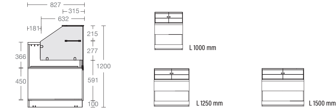
VETRINA PANETTERIA NEUTRO H1200 P825 MM BAKERY AMBIENT DISPLAY CASE H1200 D827 MM
