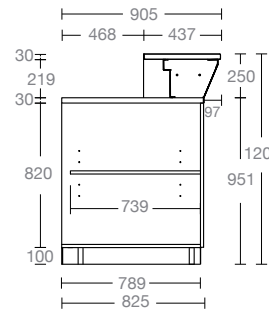
BANCO BAR NEUTRO H1200 P905MM AMBIENT BAR COUNTER H1200 P905MM
