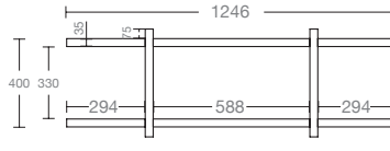
RETROALZATA BOTTIGLIERA HASTHAG P 236 HASTHAG BOTTLE COMPARTMENT D 236
