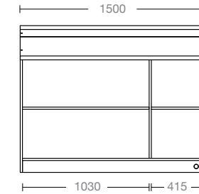
BANCO BAR NEUTRO L1500 H1200 P905MM AMBIENT BAR COUNTER W1500 H1200 P905MM
