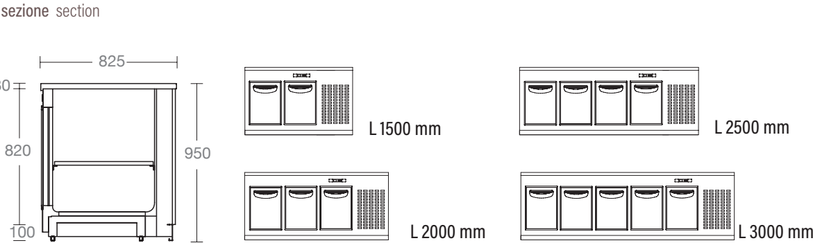
BANCO CON CELLE REFRIGERATE STATICHE E MOTORE INCORPORATO H950 P825 MM COUNTER WITH STATIC REFRIGERATED ROOMS & HERMETIC UNIT H950 D825 MM
