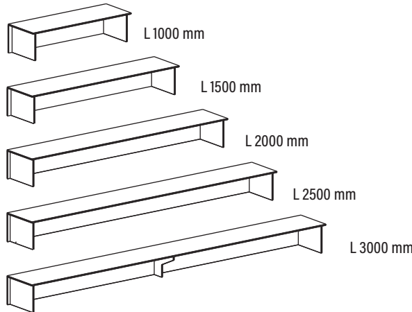
BANCO NEUTRO CON TECA IN VETRO H1200 P825 MM AMBIENT COUNTER WITH LOW GLASS H1200 D825 MM
