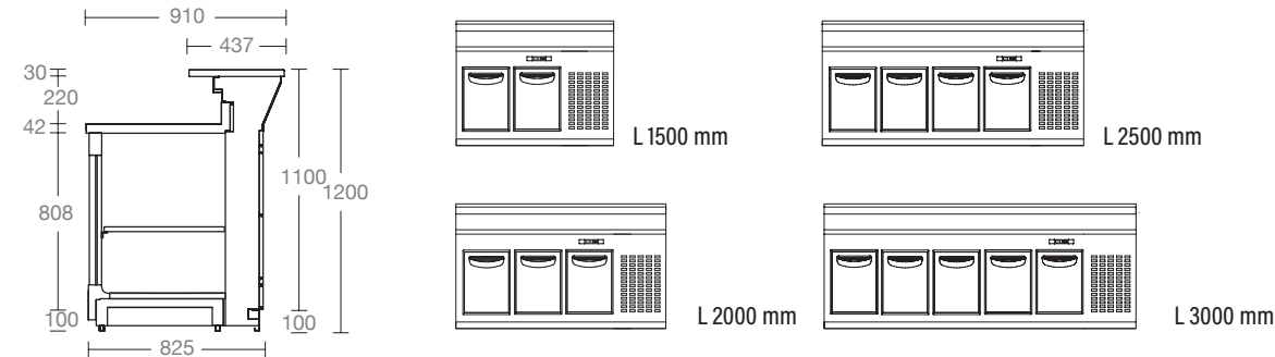
BANCO BAR CON CELLE REFRIGERATE STATICHE E MOTORE INCORPORATO H1200 P825 MM BAR COUNTER WITH STATIC REFRIGERATED ROOMS & HERMETIC UNIT H1200 D825 MM
