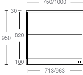
BANCO BAR NEUTRO L750/1000 H950 P825MM AMBIENT BAR COUNTER W750/1000 H950 P825MM
