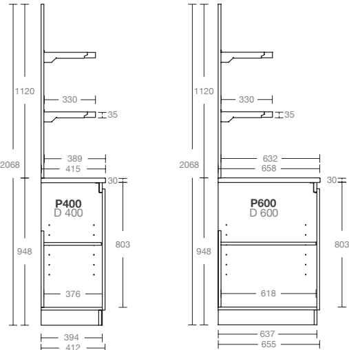
ALZATA BASE RETRO CON PIANI DRITTI WALL-MOUNTED UNIT AND BAR-BACK BASE UNIT WITH STRAIGHT SHELVES
