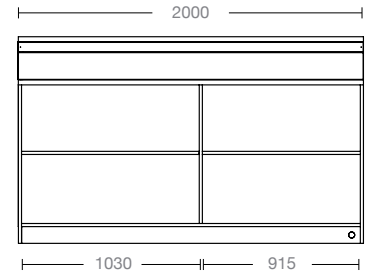
BANCO BAR NEUTRO L2000 H1200 P905MM AMBIENT BAR COUNTER W2000 H1200 P905MM
