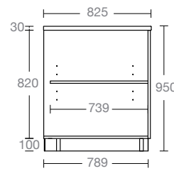
BANCO NEUTRO H950 P825MM AMBIENT COUNTER H950 P825MM
