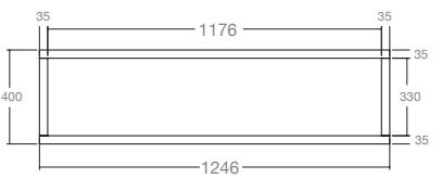
RETROALZATA BOTTIGLIERA SQUARE P 236 SQUARE BOTTLE COMPARTMENT D 236
