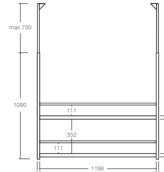
MENSOLA PORTA BOTTIGLIE A SOFFITTO CEILING BOTTLE COMPARTMENT
