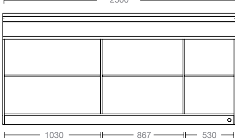
BANCO BAR NEUTRO L2500 H1200 P905MM AMBIENT BAR COUNTER W2500 H1200 P905MM
