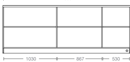
BANCO BAR NEUTRO L2500 H950 P825MM AMBIENT BAR COUNTER W2500 H950 P825MM
