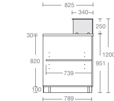
BANCO NEUTRO CON TECA IN VETRO H1200 P825 MM AMBIENT COUNTER WITH LOW GLASS H1200 D825 MM
