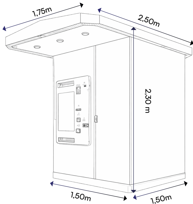
DIMENSIONS OF THE SMART PIZZA JULIA VENDING MACHINE
