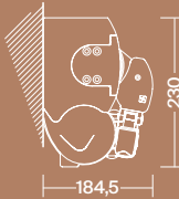
Wall installation 0° - 85° Installation murale 0° - 85°
