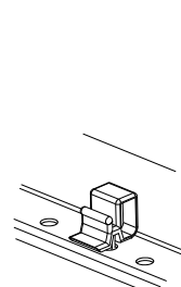
Mounting clip PR7-MCB at the bottom of SP7
