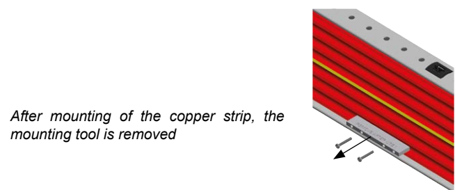
Isolation strip on which copper strip is applied using PR-ISO mounting tool
