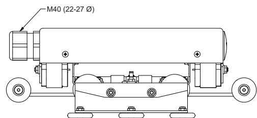
Mounting set PCT7-SB
