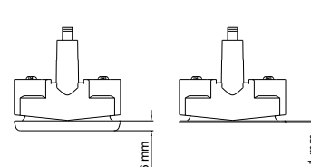
Inspecting the contact surface of the carbon brush
