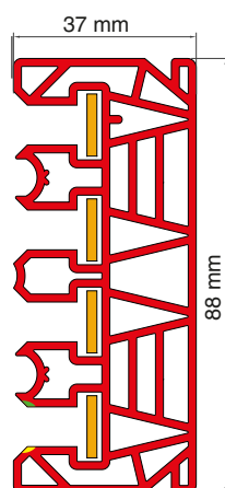
Housing PR4 with copper conductors
