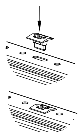
Mounting clip PR7-MCT on top of SP7
