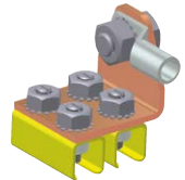
Connector C-LC400 with 2 clamps LC200
