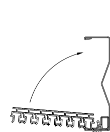
Mounting PR7 after placing mounting clips PR7-MCB
