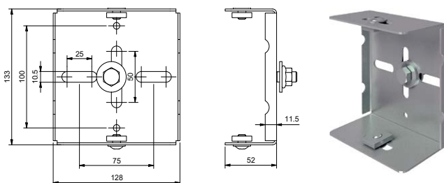
Mounting bracket SP4-MB
