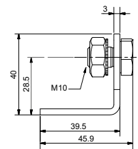
Connector C(J)-LC400 side view
