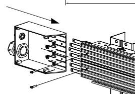
Mounting end feed box to PR7 housing)
