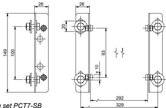
Mounting set PCT7-SB
