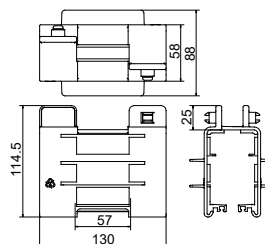
Mounting RC-LCH
