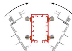
Mounting RC-LCH
