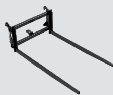
Pallet fork carriage for poultry containers
