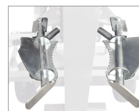
Log holding arm
