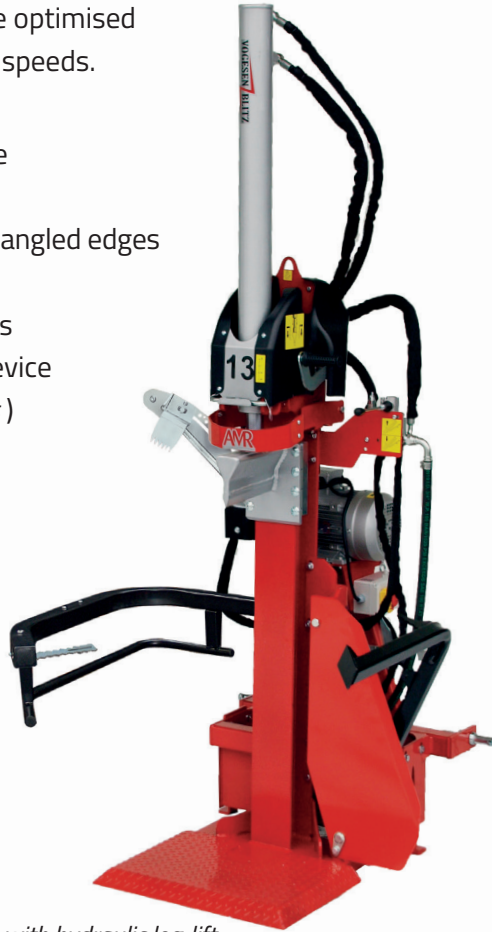
VPE13 with hydraulic log-lift
